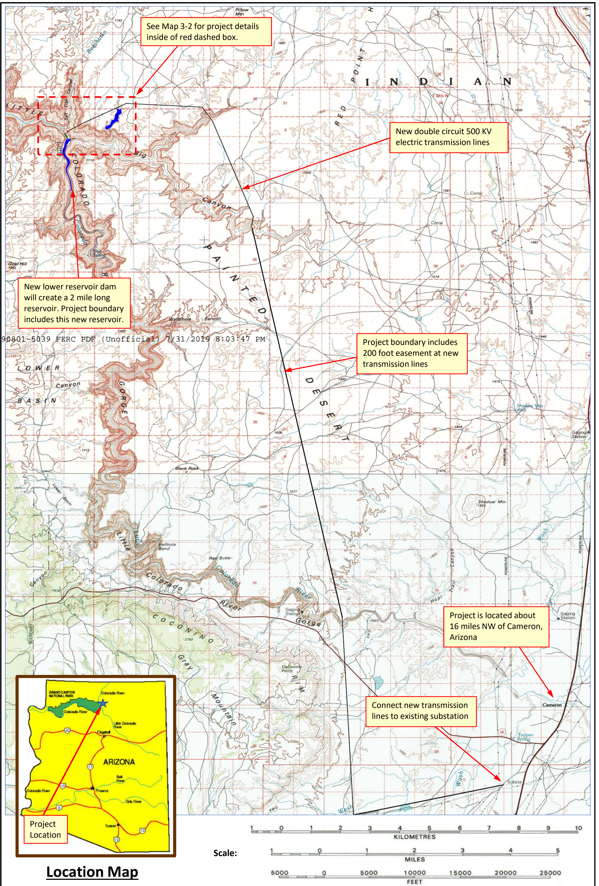
Exhibit 3-1 - Navajo Nation Pumped Storage Project Conceptual Design Map 1
